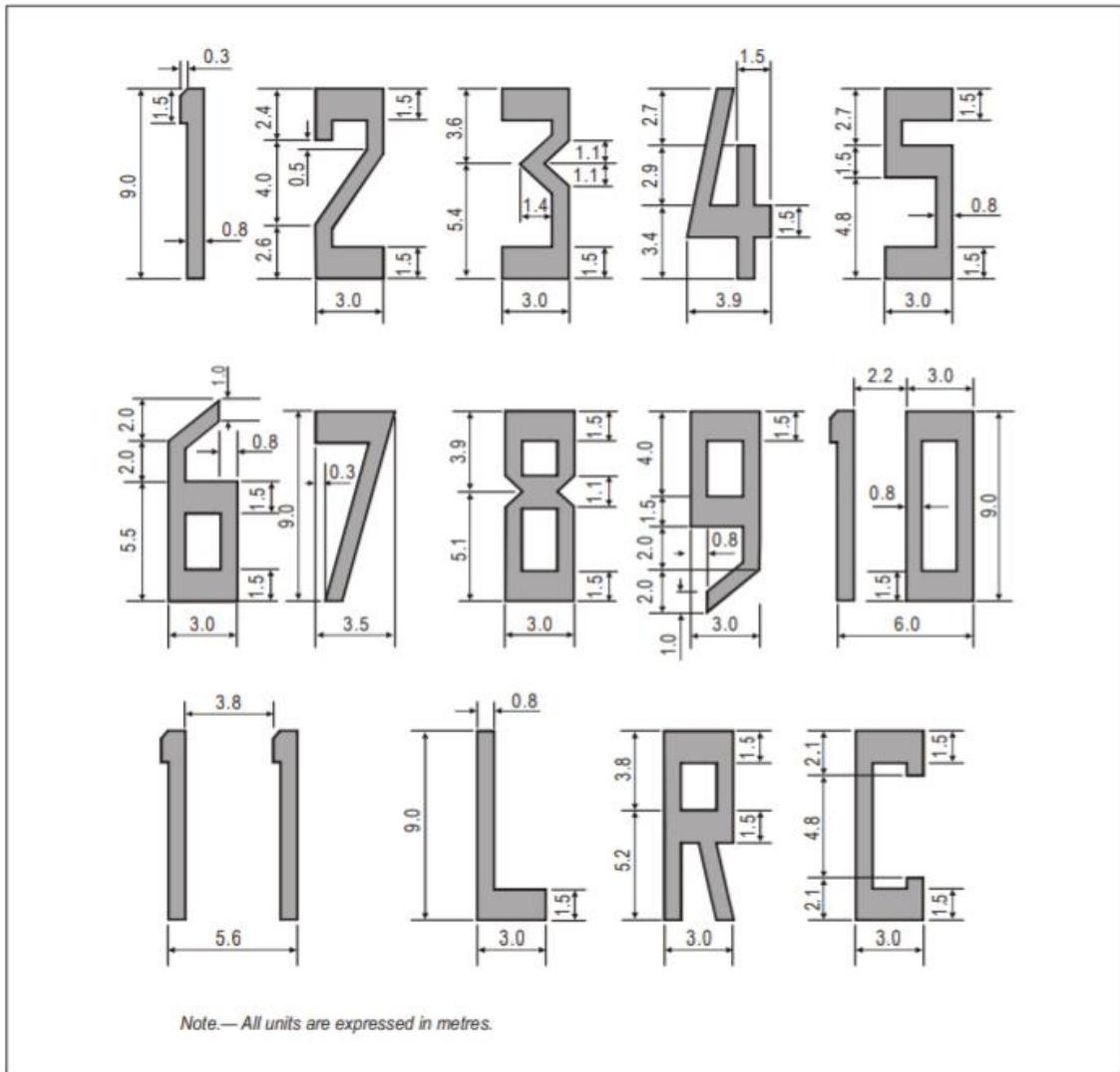
Figure 5-3. Form and Proportions of Numbers and Letters for Runway Designation Markings
