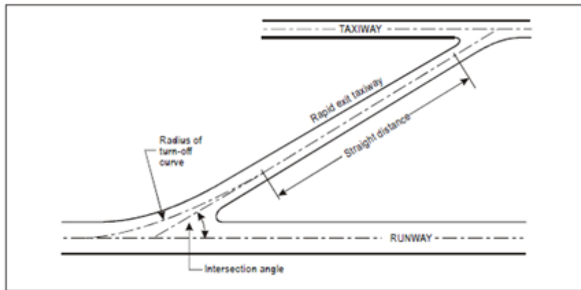
Rapid Exit Taxiway
