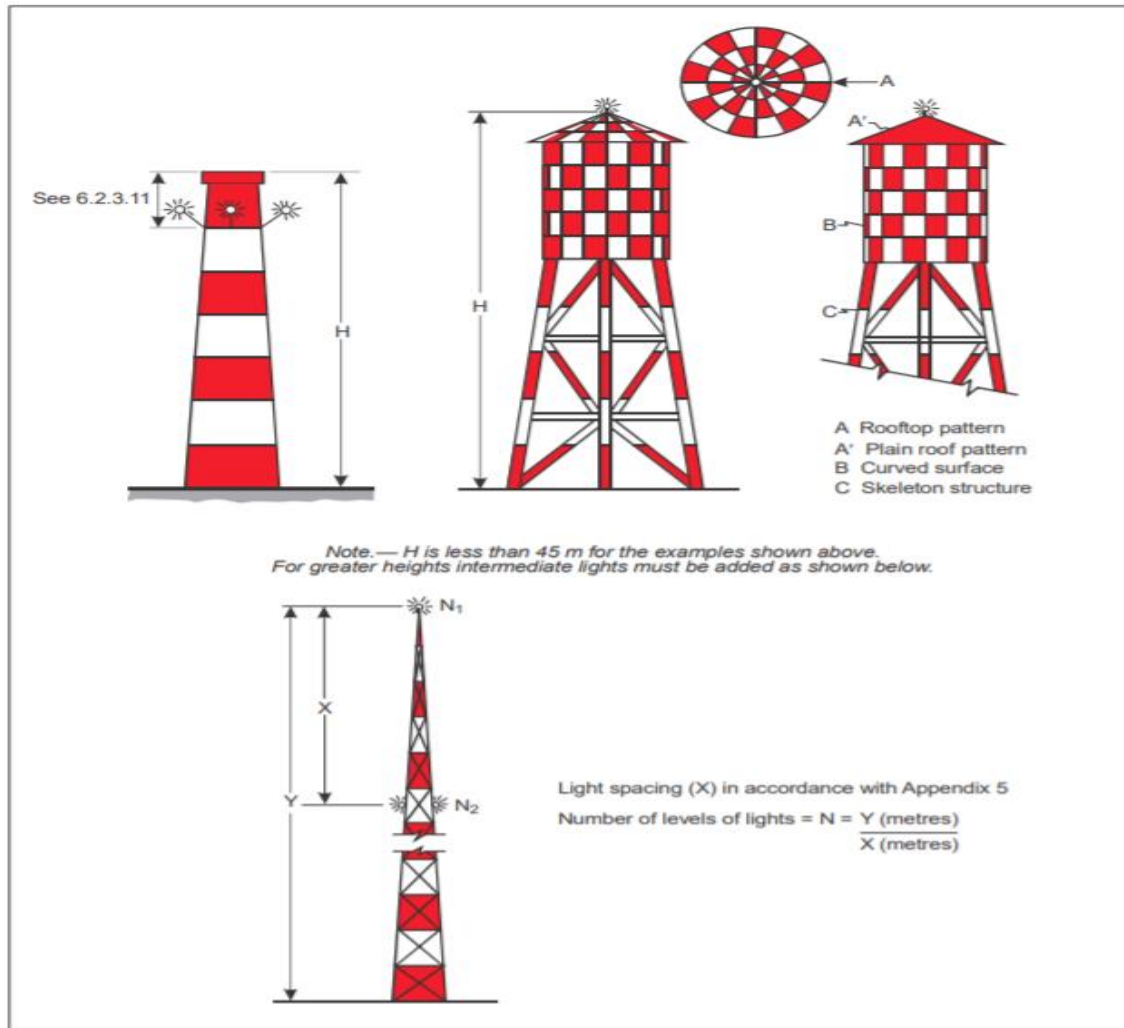
Figure 2: Marking and Lighting of Tall Structures
