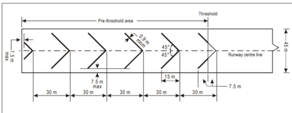
Figure 4. Pre-Threshold Marking
