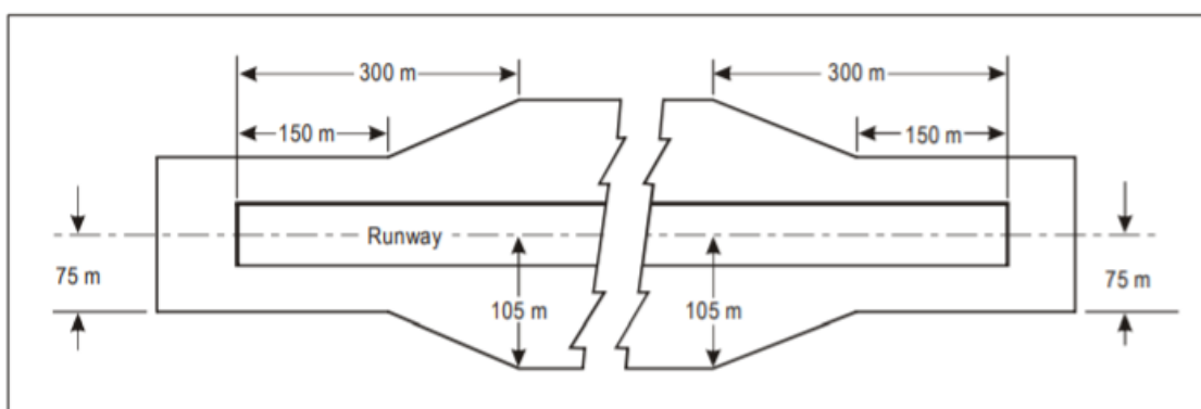
Figure B-4. Graded Portion of a Strip Including A Precision Approach Runway Where The Code Number Is 3 or 4
