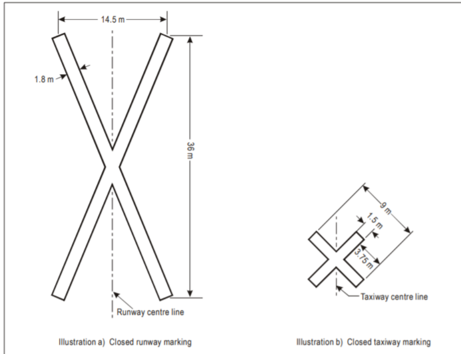
Figure 3. Closed Runway and Taxiway Markings
