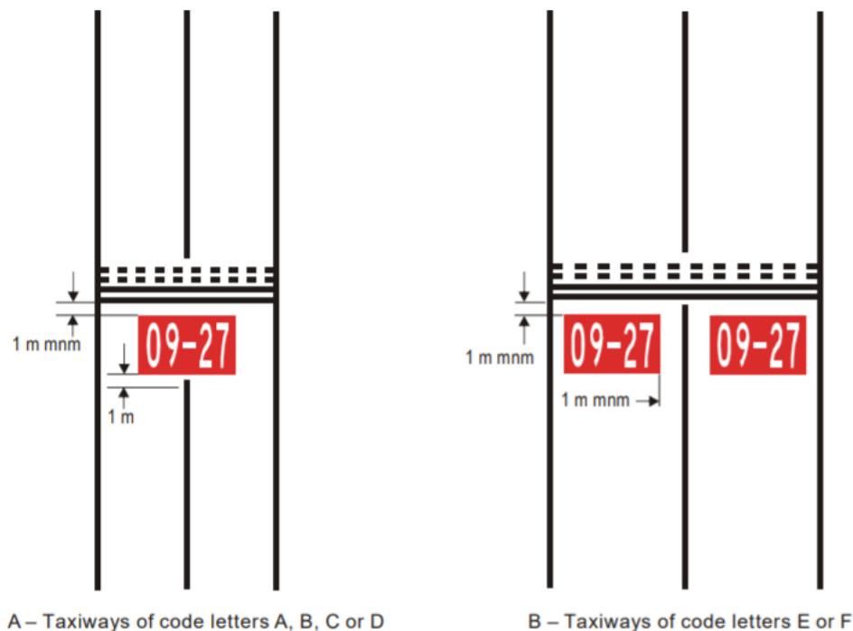
Figure 5-10. Mandatory Instruction Marking
