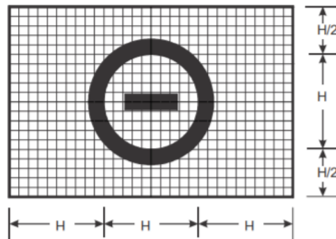
Figure A4-3. Runway vacated and NO ENTRY signs
