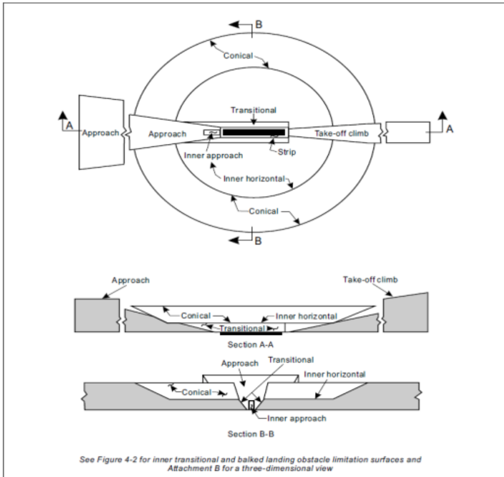
Figure 4-1. Obstacle limitation surfaces
