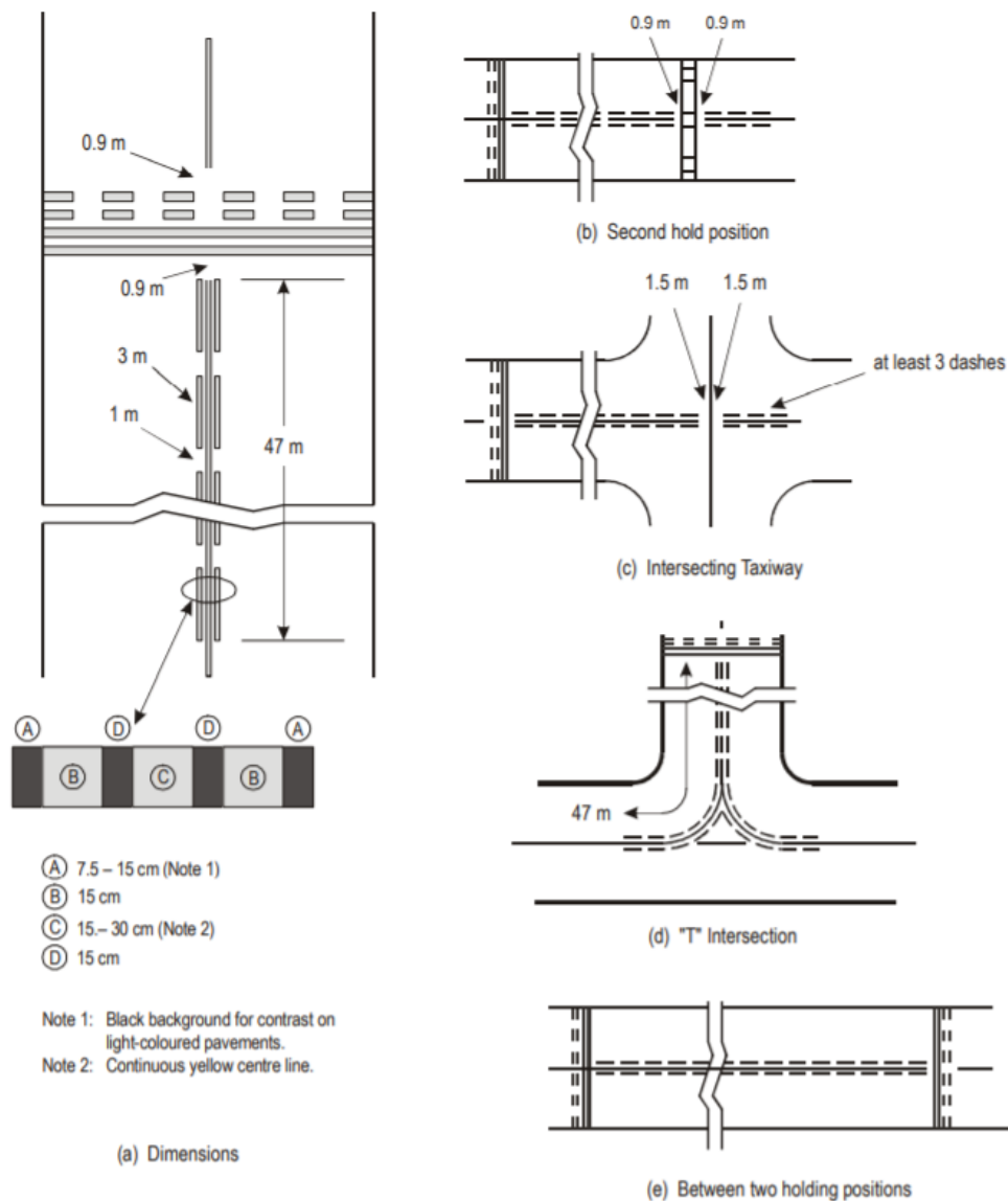
Figure 5-7. Enhanced Taxiway Centre Line Marking
