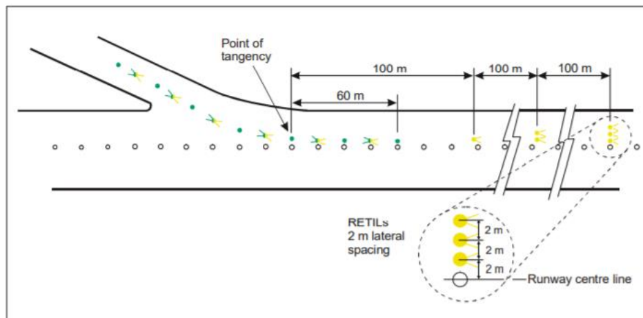
Figure 5-25. Rapid Exit Taxiway Indicator Lights (RETILs)
