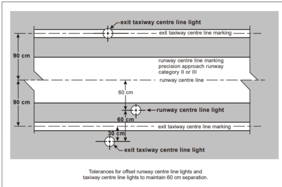
Figure 5-27. Offset Runway and Taxiway Centre Line Lights
