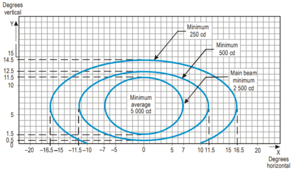
Figure A2-1. Isocandela Diagram for Approach Centre Line Light and Crossbars (White Light)
