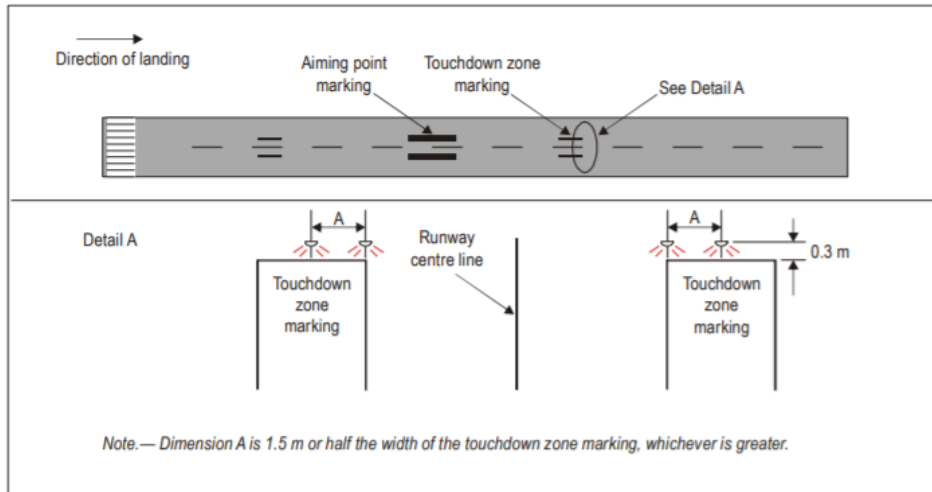
Figure 5-24. Simple Touchdown Zone Lighting
