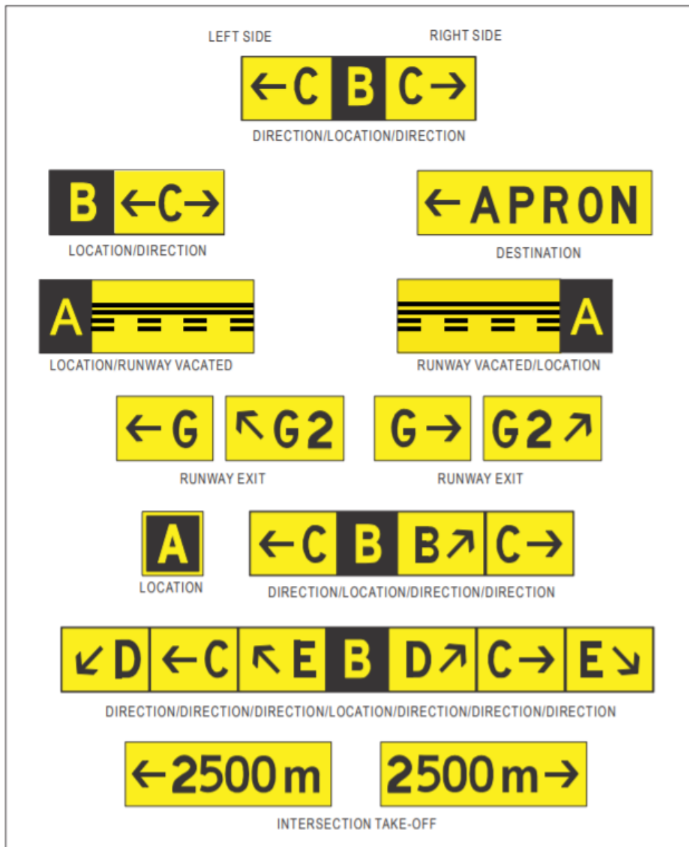
Figure 5-31. Information Signs
