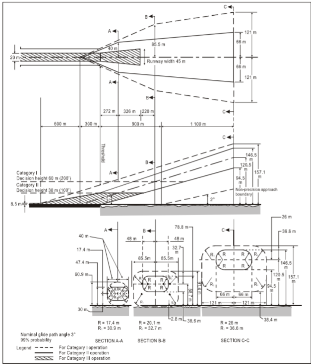
Figure A-6. Flight Path Envelop to Be Used for Lighting Design for Category I, II and III Operations
