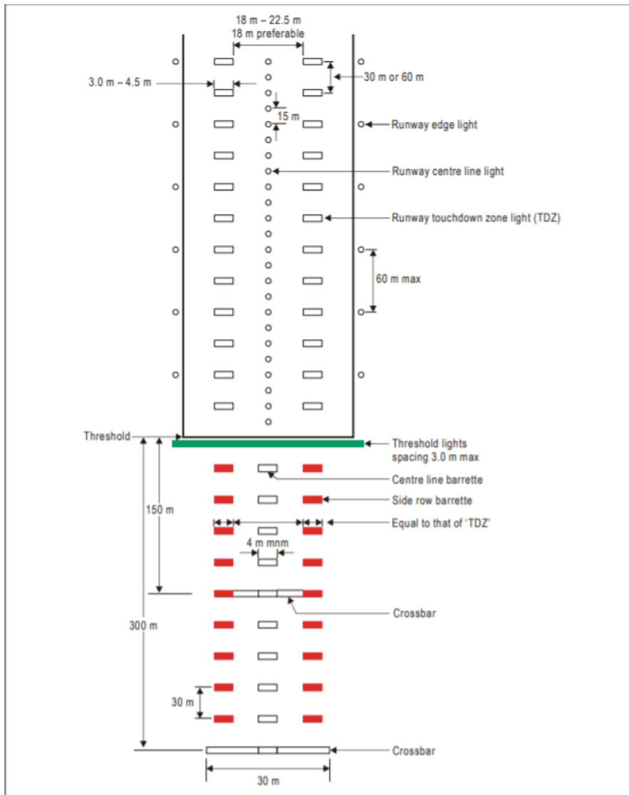
Figure 5-14. Inner 300 m Approach and Runway Lighting for Precision Approach Runways, Categories II and II
