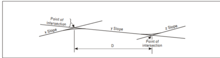
Figure A-2: Profile on Center Line of Runway
