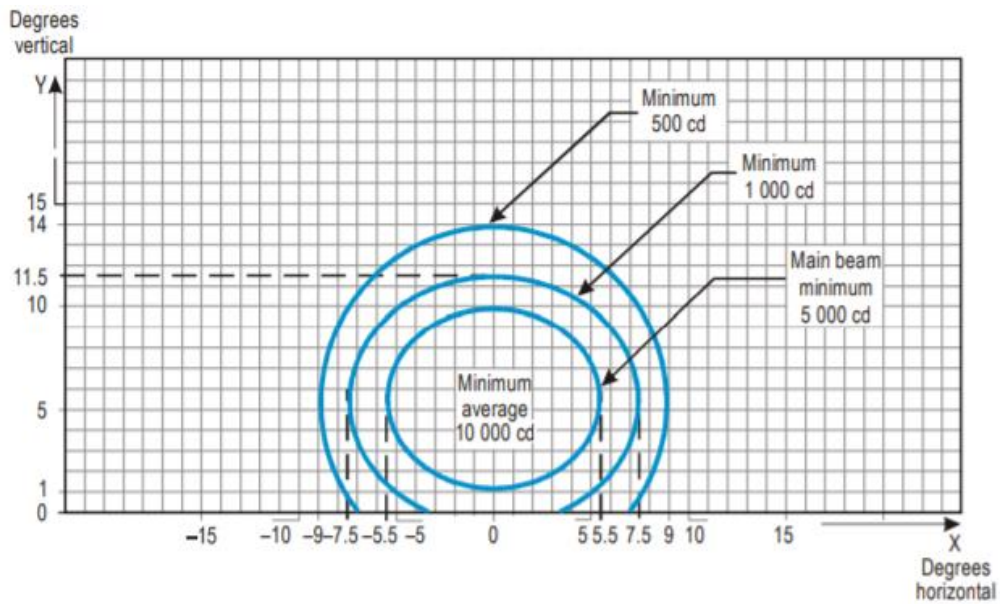
Figure A2-2. Isocandela Diagram for Approach Side Row Light (Red Light)
