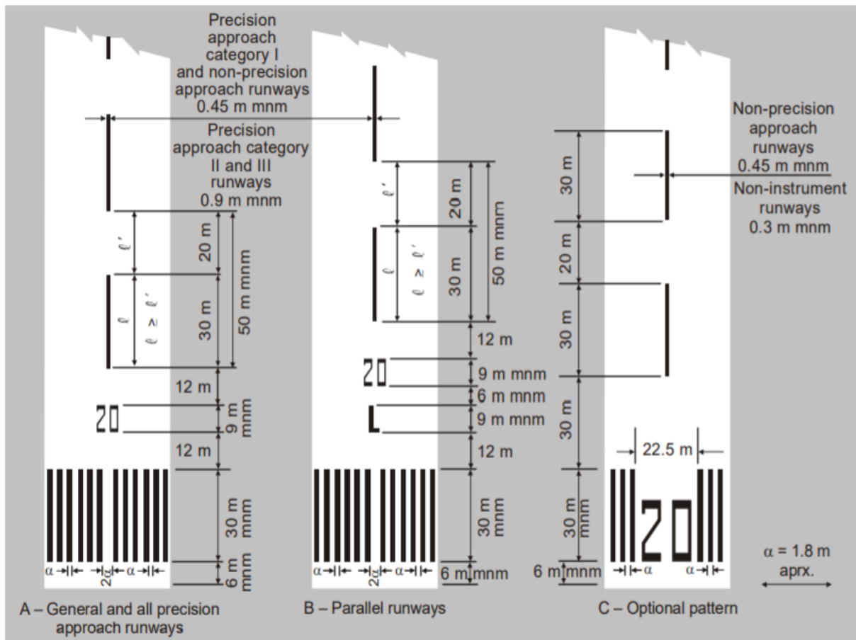
Figure 5-2. Runway designation, centre line and threshold markings
