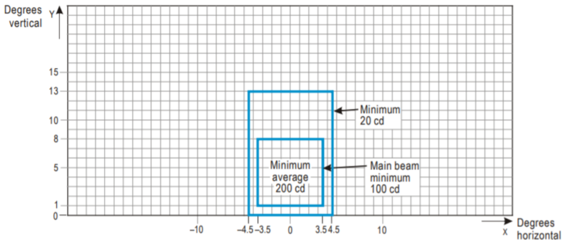
Figure A2-12. Isocandela Diagram for Taxiway Center Line (15 M Spacing), No-Entry Bar and Stop Bar Lights in Straight Sections Intended for Use in Runway Visual Range Conditions of Less Than a Value Of 350 M Where Large Offsets Can Occur and For Low-Intensity Runway Guard Lights, Configuration B
