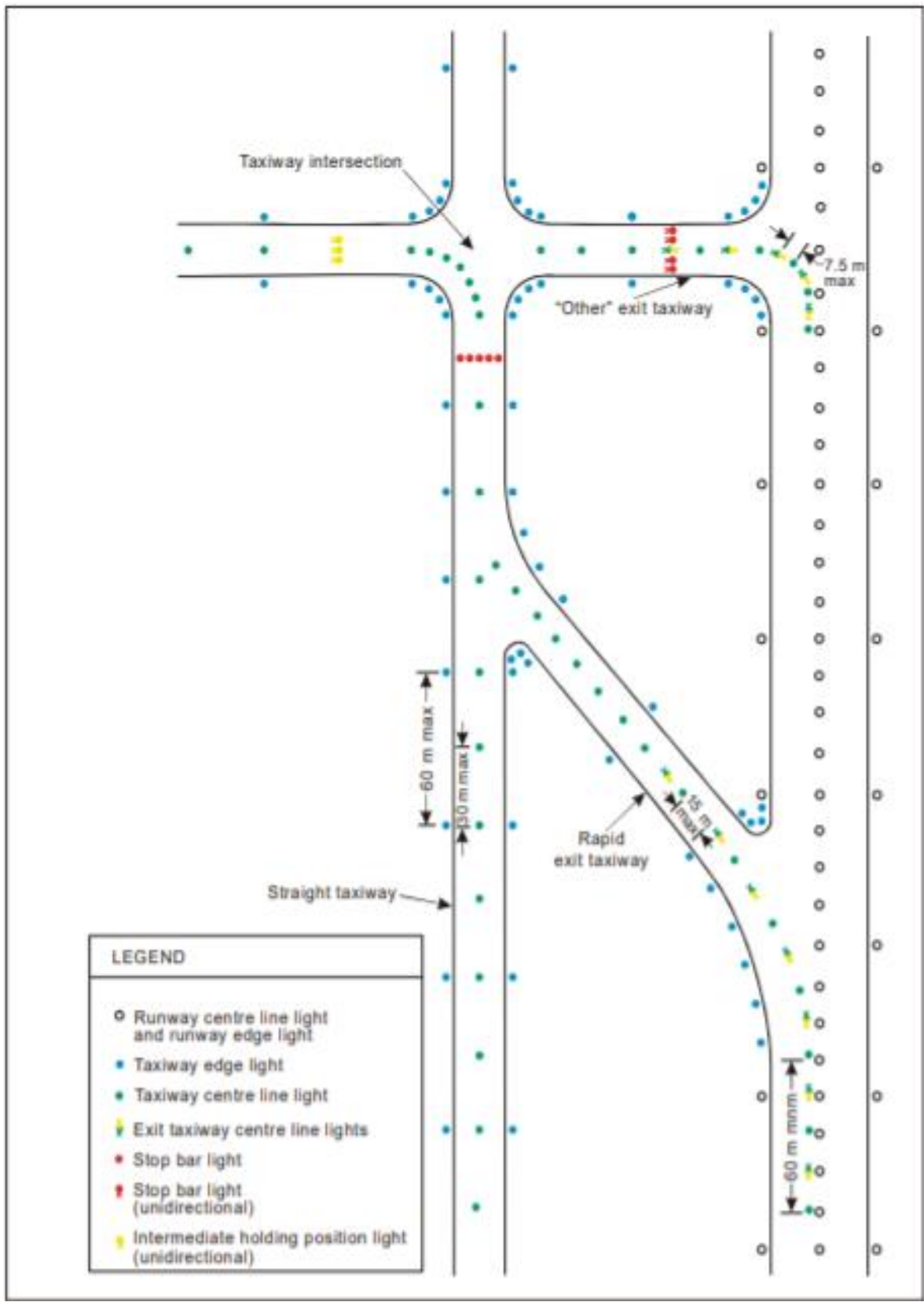
Figure 5-26. Taxiway Lighting
