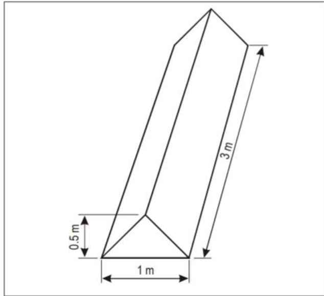
Figure 5-34 Boundary Markers
