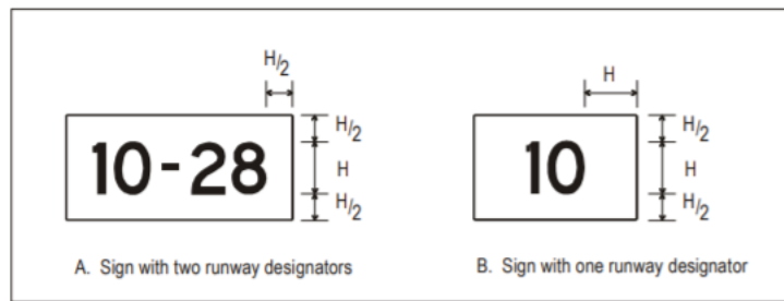
Figure A4-3. Sign dimensions
