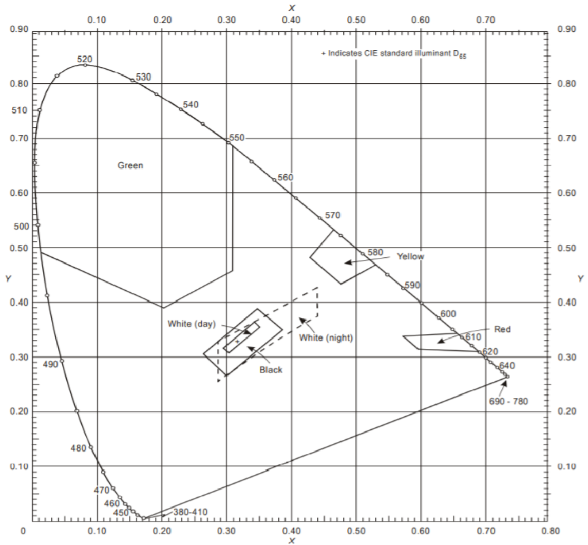
Figure A1-4. Colours of Luminescent or Trans Illuminated (Internally Illuminated) Signs and Panels
