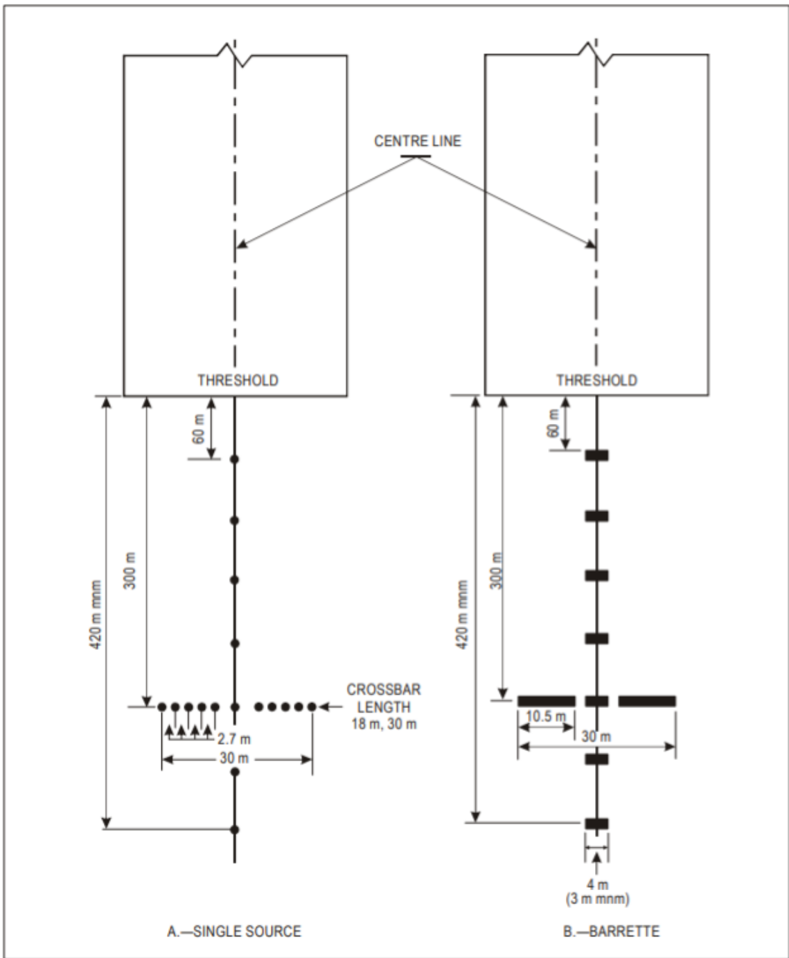
Figure A-7. Simple Approach Lighting System
