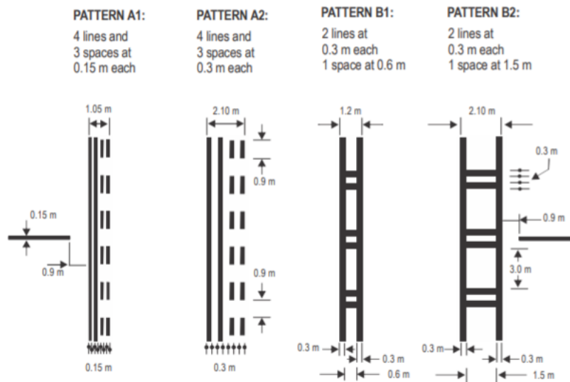
Figure 5-8. Runway-Holding Position Markings
