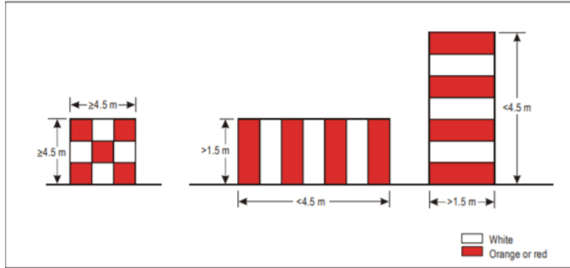
Figure 1. Basic Marking Patterns
