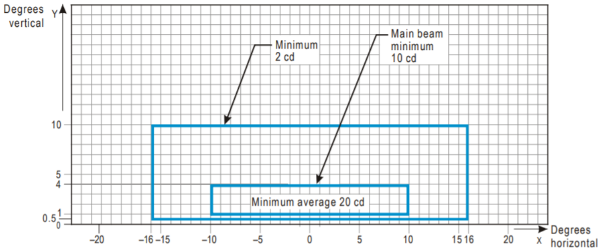
Figure A2-14. Isocandela Diagram for Taxiway Center Line (7.5 M Spacing), Rels, No-Entry Bar and Stop Bar Lights in Curved Sections Intended for Use in Runway Visual Range Conditions of Less Than a Value Of 350 M
