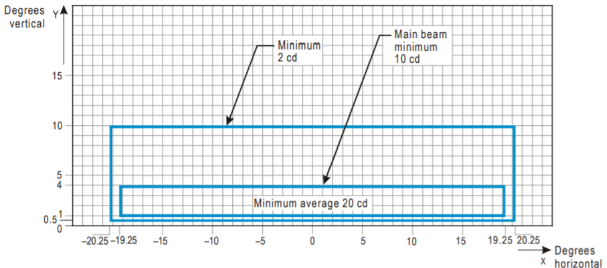
Figure A2-15. Isocandela Diagram for Taxiway Center Line (30 M, 60 M Spacing), No-Entry Bar and Stop Bar Lights in Straight Sections Intended for Use in Runway Visual Range Conditions Of 350 M or Greater
